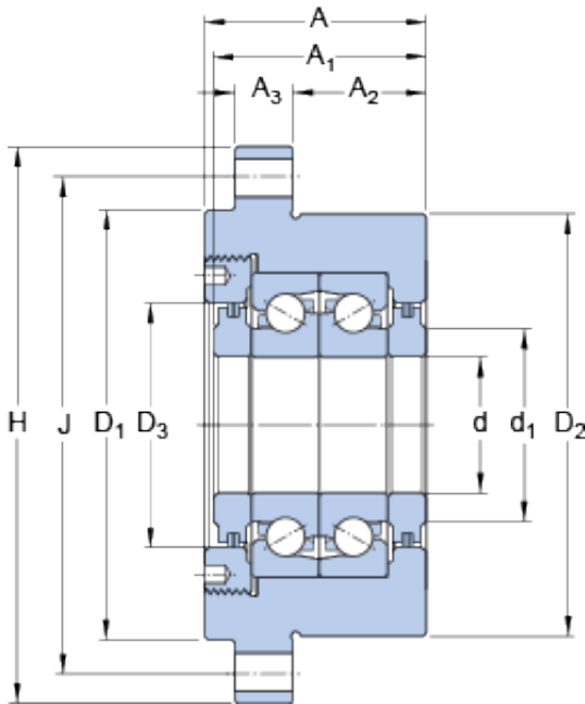
FBSA 205/DF Bearing 2D drawings and 3D CAD models
